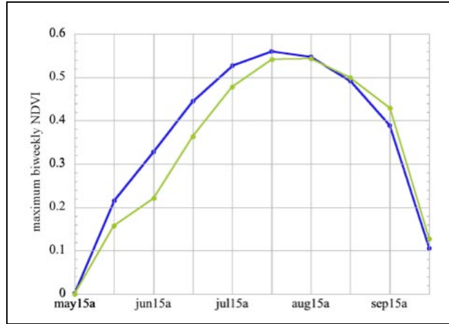
Figure 6 Climatological seasonal cycle (1982-2006) of semimonthly maximum NDVI in the Beaufort (blue) and W. Kara (green) regions.
