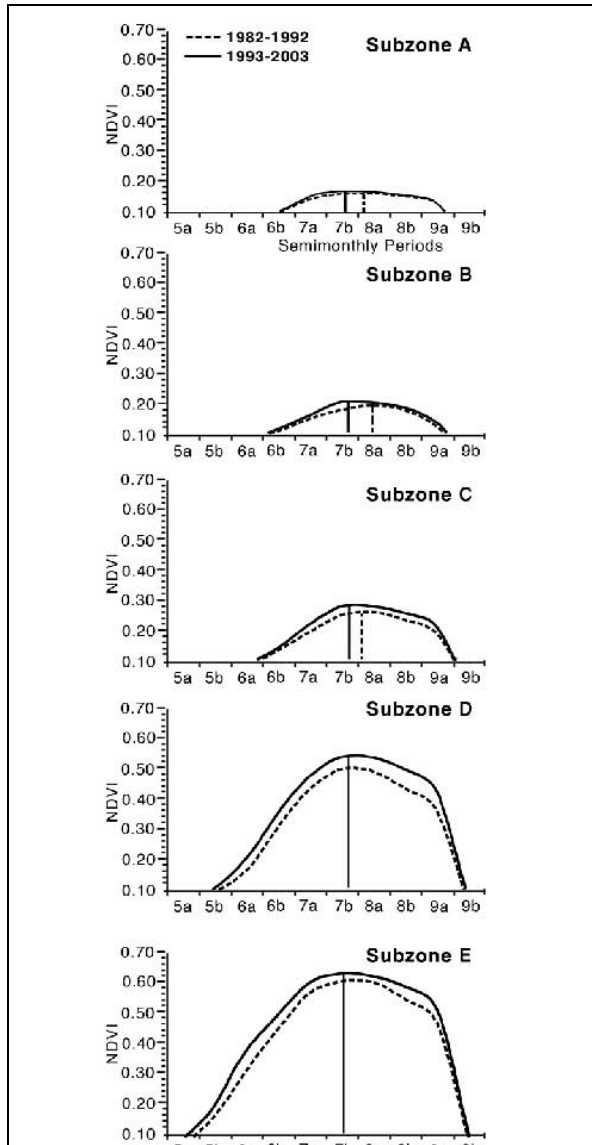
Figure 5. Integrated NDVI curves for 1982-1992 (dashed lines) and 1993-2003 (solid lines) within the five bioclimate subzone in the tundra zone of Arctic Canada. The x-axes show semi-monthly time periods, from which the maximum NDVI values were extracted. There has been an increase in maximum NDVI within all five subzones. Vertical lines show the shift toward an earlier maximum NDVI within the High Arctic subzones (A, B, and C). An earlier onset of greening has occurred only in the Low Arctic (subzones D and E). Modified from Jia et al. 2008 in review.
