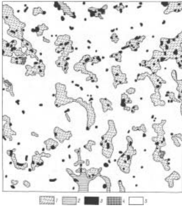
Fig. 16.34. Sporadically spotted type of horizontal structure in a Dryas punctata heath on a fell-field in Maria Pronchishcheva Bay, Taymyr. 1, Dryas punctata ; 2, Salix polaris ; 3, Novosieveria glacialis ; 4, moss turf of Dicranum elongatum and Polytrichum strictum ; 5, fell-fields with crustose lichens. Sample plot 10x10 m.
