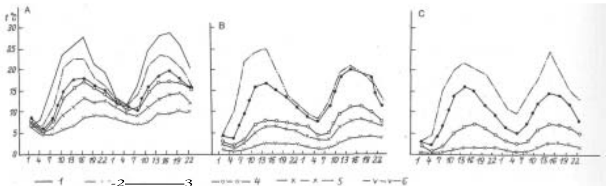
Fig. 16.48. Daily course of soil temperature in different elements of nanorelief in a frost-boil Betula «««a-sedge-moss community in the southern tundra subzone at Kresty, Taymyr, June 1976. A, patch of bare ground; B, rim; C, trough; 1, air; 2, soil or moss surface; 3, depth 2 cm; 4, depth 5 cm; 5, depth 10 cm; 6, depth 15 cm.
