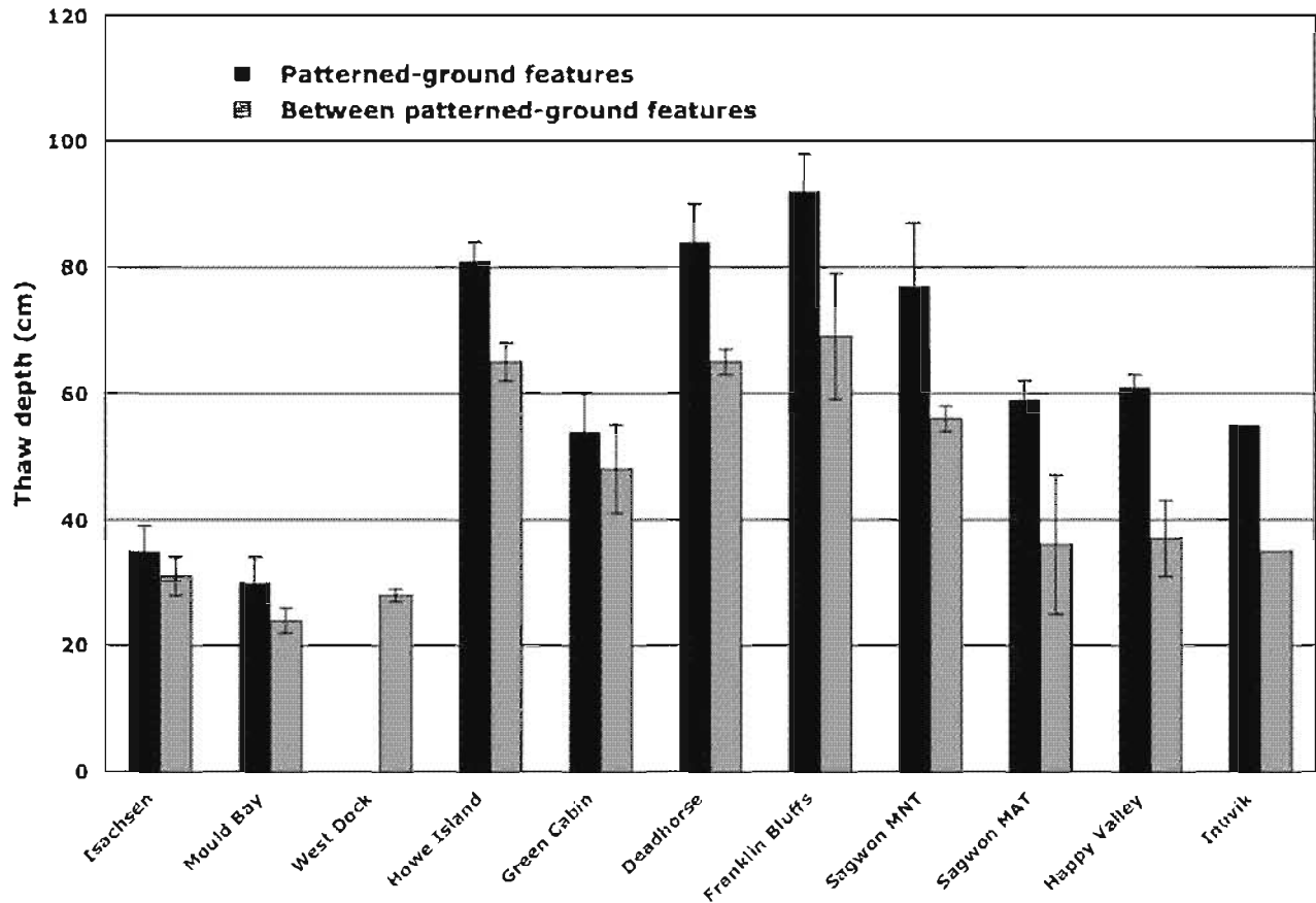
Figure 9. Mean thaw-depth ( \pm s.d.) along the NAAT in late August 2006. Data are from the vegetation study plots of the dominant vegetation types on and between PGFs of zonal sites at each location; n = 5–7 except at Inuvik where n = 1.
